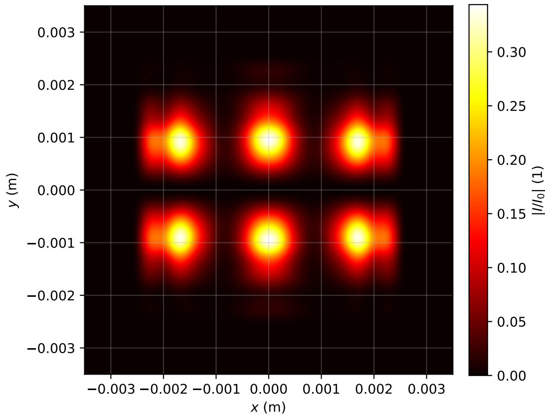
Intensity profile I(x, y, z = 3.981)/I_0 , P_{in}=3.0P_{cr} , artificial time
